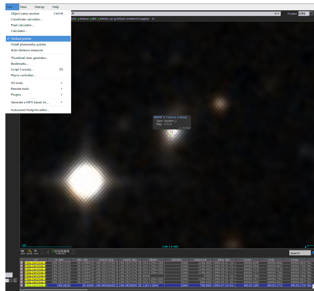
Figure 14: How to enable and operate the SIMBAD pointer in Aladin.
