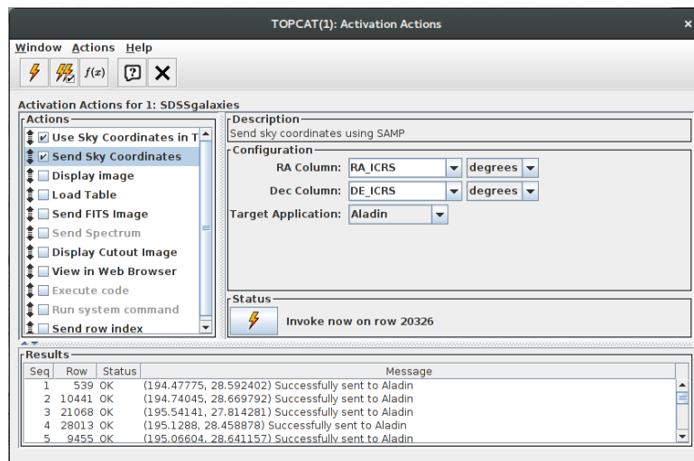
Figure 5: Setting up activation actions in TOPCAT.
