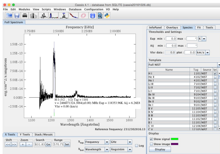
Figure 13: Spectrum with CASSIS. The the blue, dotted line and the green dash mark the location of the \text{Ly}\alpha line at a line of sight velocity of 0.0 \text{ km s}^{-1}
