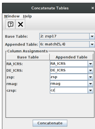
Figure 8: Concatenating with TOPCAT.
