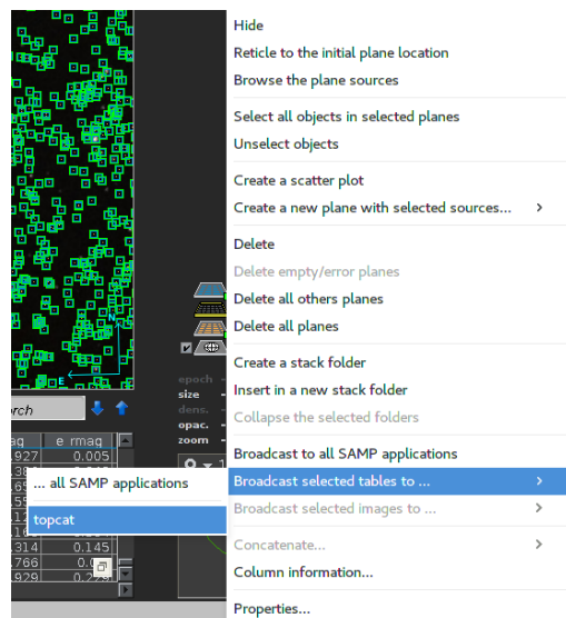
Figure 4: Broadcasting the filtered catalogue to TOPCAT.
