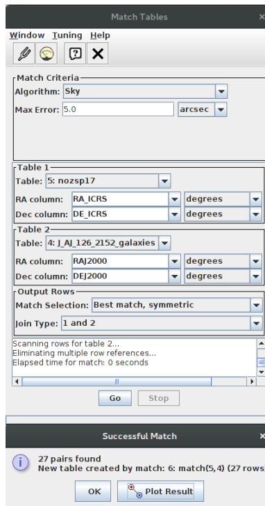
Figure 7: X-matching with TOPCAT.
