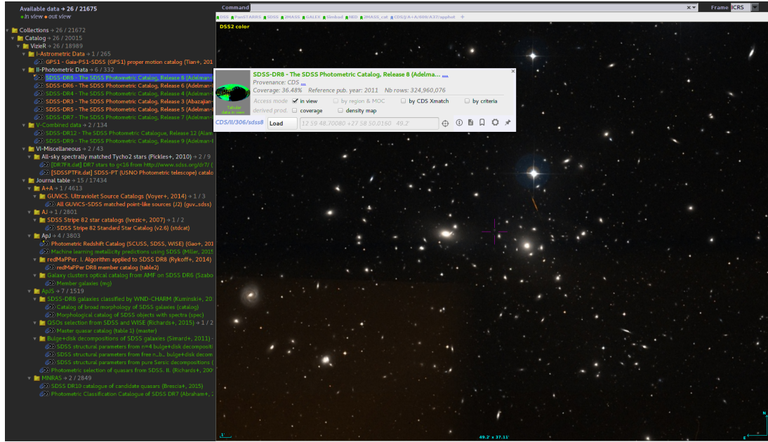
Figure 2: The Aladin DATA TREE when filtered to "SDSS" resources in "large catalogues". Green resources have entries in the area of the sky that is currently shown in the main viewing window, orange ones not. The grey pop-up window allows you to load the data in different ways, e. g. load all data within the field of view or filter the catalogue by MOC.
