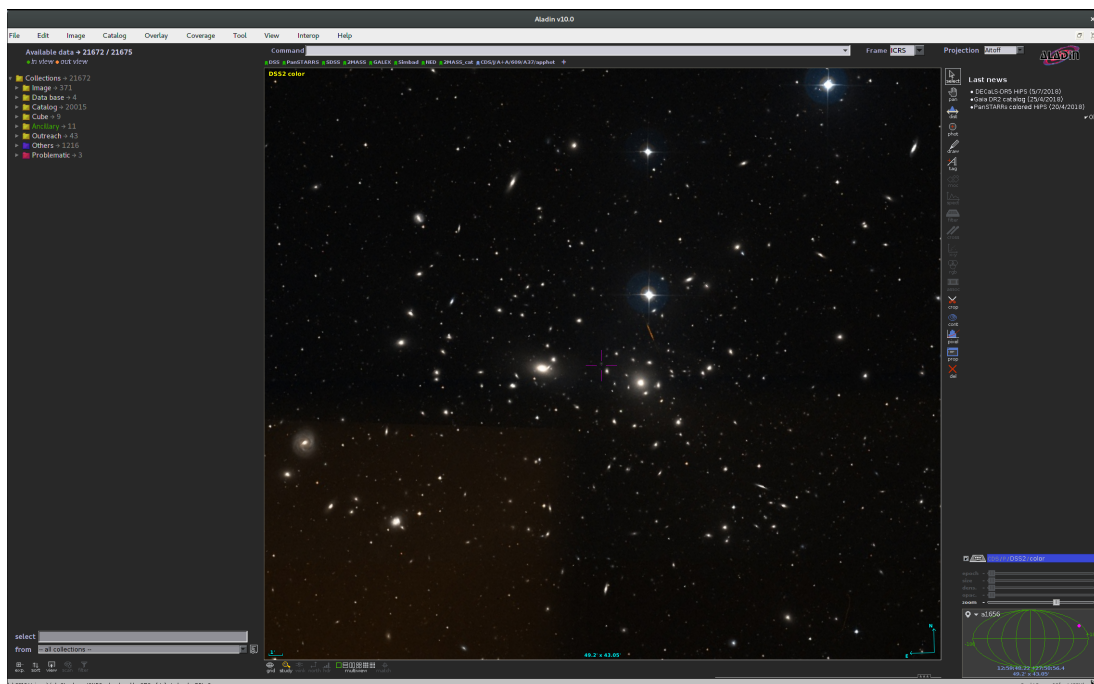
Figure 1: Abell 1656 (Coma Cluster) in Aladin
