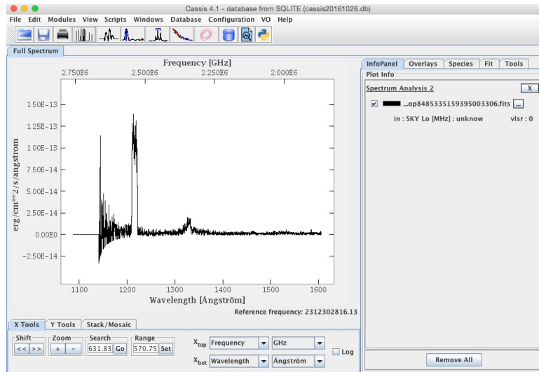
Figure 12: Visualisation of the spectrum with CASSIS.
