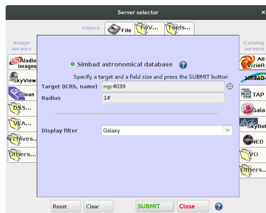
(b) The SERVER SELECTOR window: here SIMBAD has been queried for galaxies within 14 arcmin around NGC 4093.
