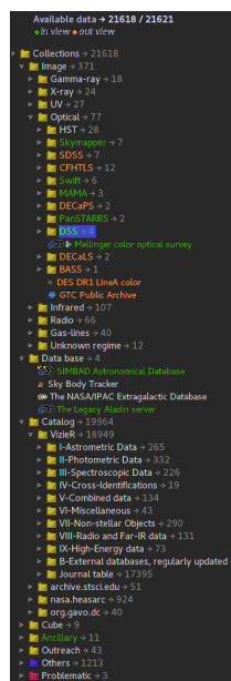
(a) The DATA TREE: green entries are available for the sky region currently visible in the main viewing window (not shown).
